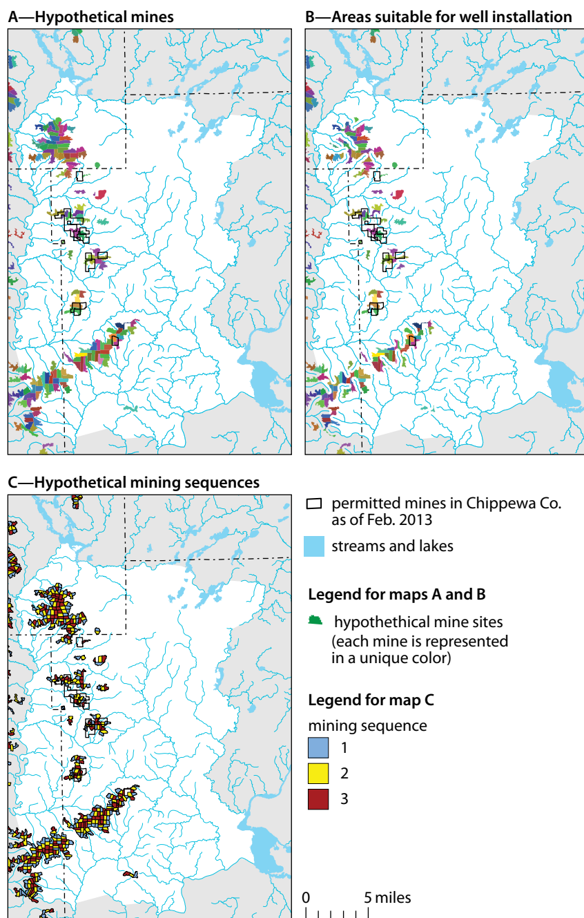
Figure 34. Mine buildout maps showing (A) the minable Woneewoc resource segmented into 155 hypothetical mines of approximately 150 minable acres each, (B) segments with well locations at least 1,200 feet from a stream, and (C) hypothetical three-step mine development sequences.
