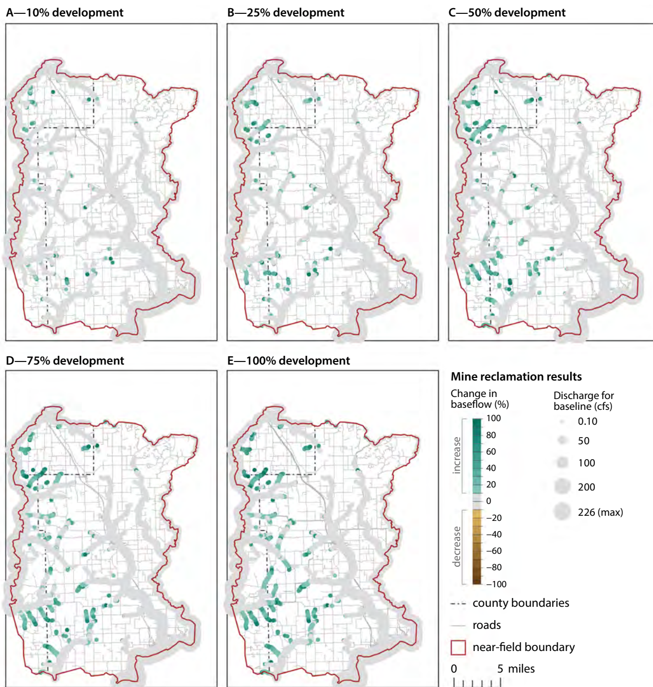
Figure 36. Percent baseflow change due to long-term prairie reclamation following simultaneous mine development of the minable Wonewoc resource.
