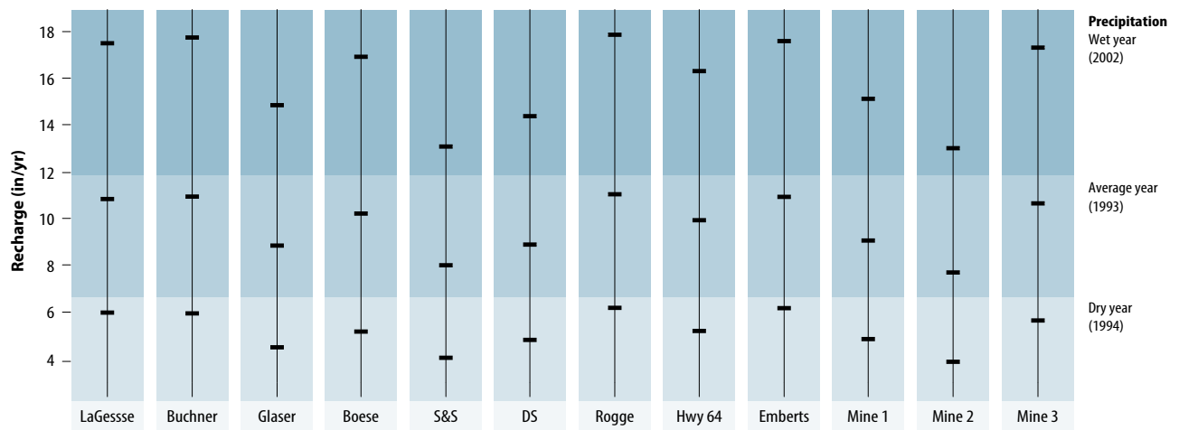
Figure 18. SWB-estimated recharge during wet, average, and dry years at 12 mine sites under pre-mining land use. Example shows differences from site to site and from year to year.
