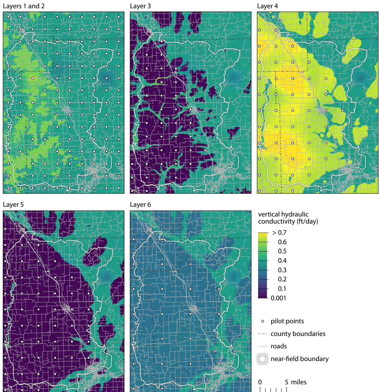
Figure 27. Calibrated vertical hydraulic conductivity, by model layer. Layers 1 and 2 are combined because they have the same hydraulic conductivity values. Layer thickness is 2 feet wherever a unit is absent within a model layer.
