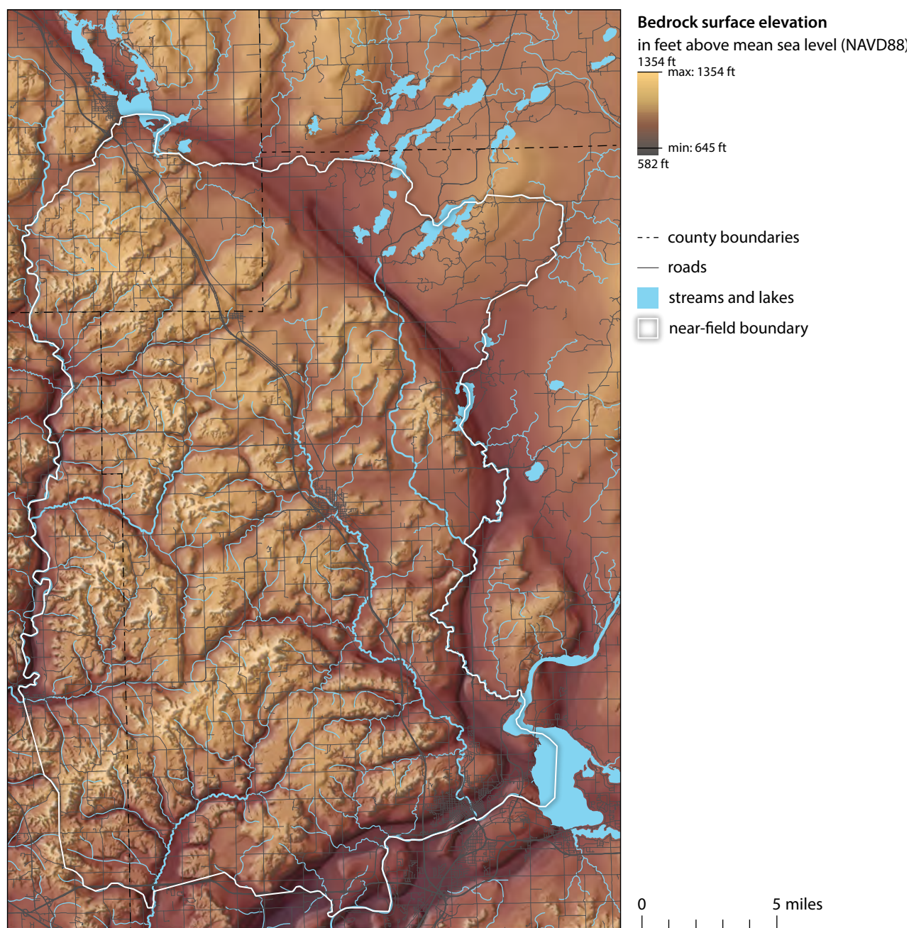
Figure 5. Bedrock surface elevation.
