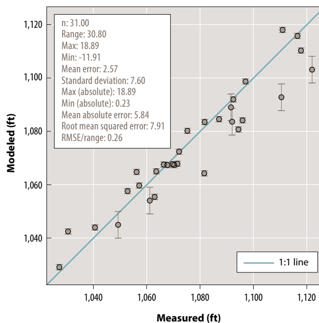
Figure 29. Mine residuals.
