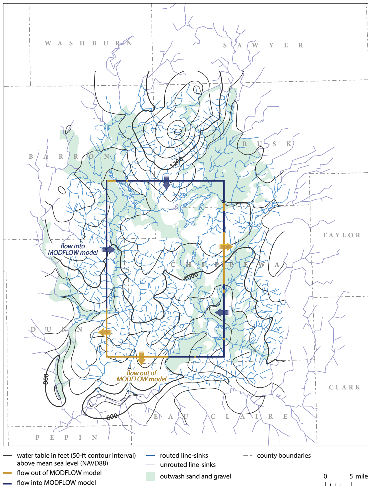
Figure 19. GFLOW model line-sinks showing direction of groundwater flow across model boundaries.
