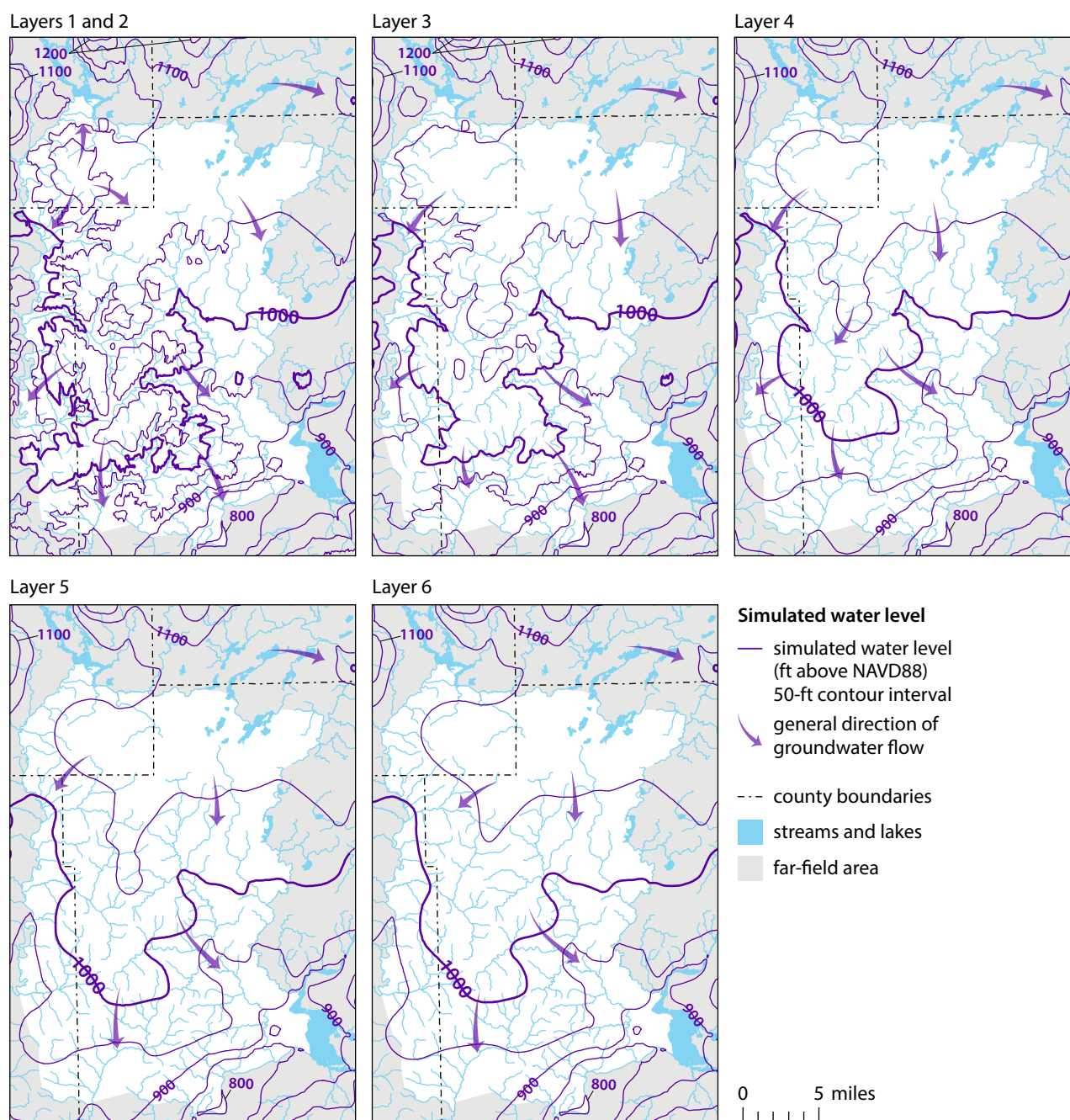
Figure 33. Simulated water levels, by model layer.
