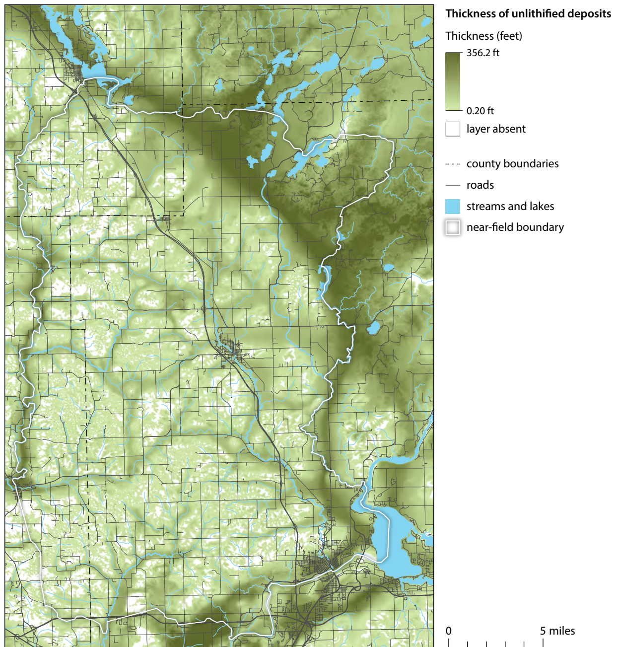
Figure 4. Thickness of unlithified deposits.
