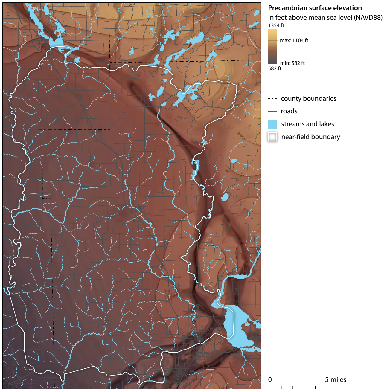
Figure 6. Precambrian surface elevation.
