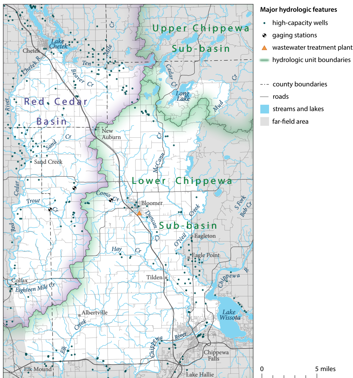
Figure 3. Major hydrologic features of the study area.
