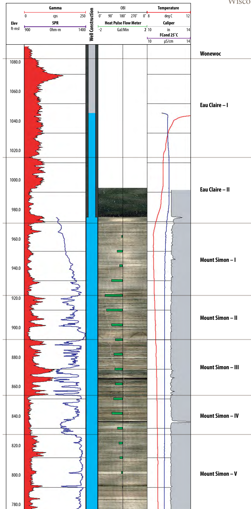
Figure 8. Hydrostratigraphic units from a borehole geophysical log. (See fig. 2 for additional information about this log.)
