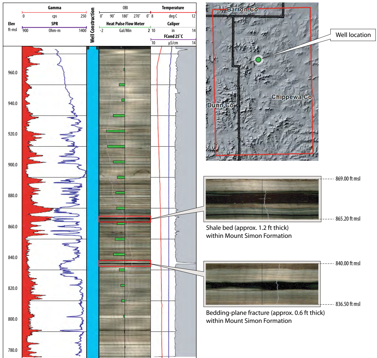
Figure 2. Example borehole geophysical log. High-resolution imagery from the optical borehole imaging (OBI) tool reveals a shale bed and a bedding-plane fracture within the Mount Simon Formation. From the Superior Silica Sands Culver mine (WGNHS ID 9000341).
