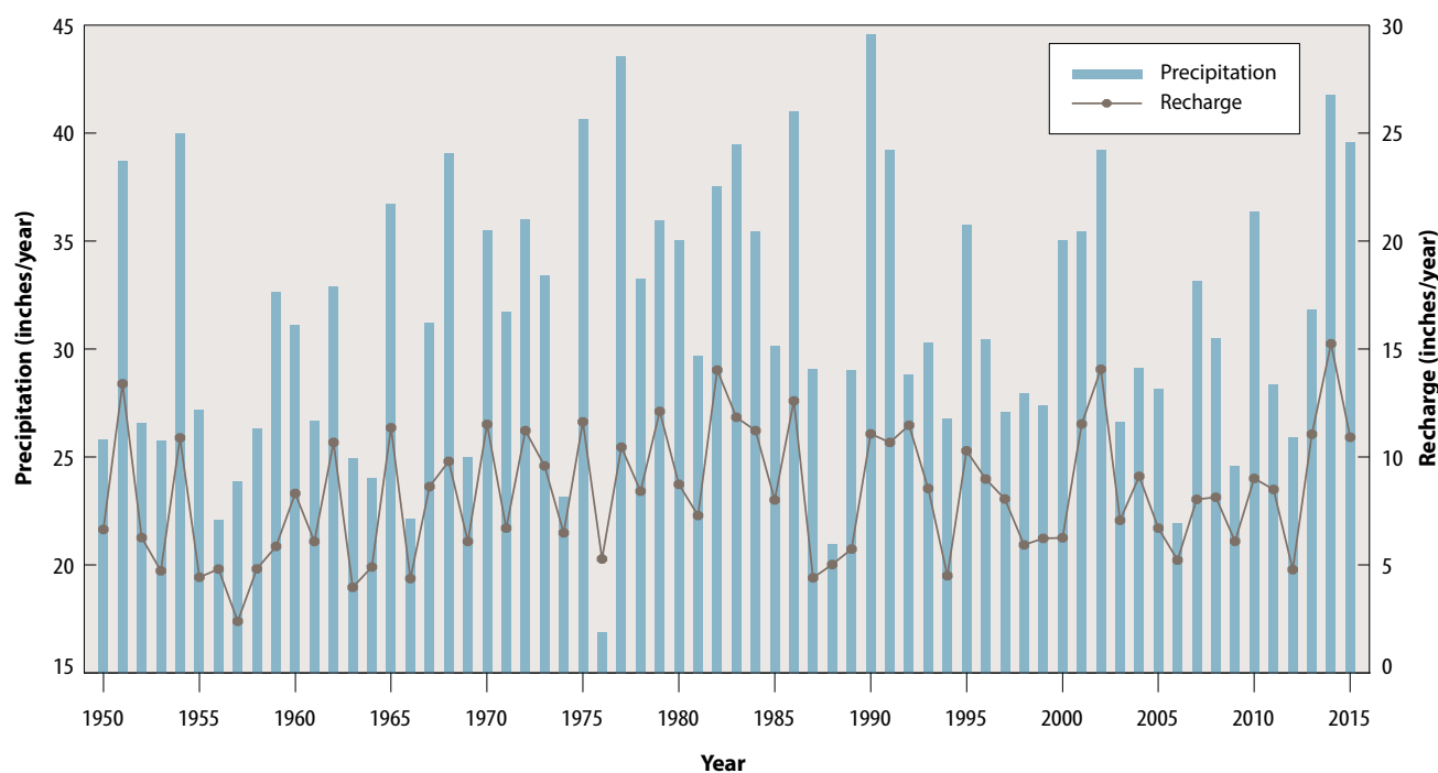
Figure 15. Precipitation and SWB-estimated recharge for study area, 1950–2015.
