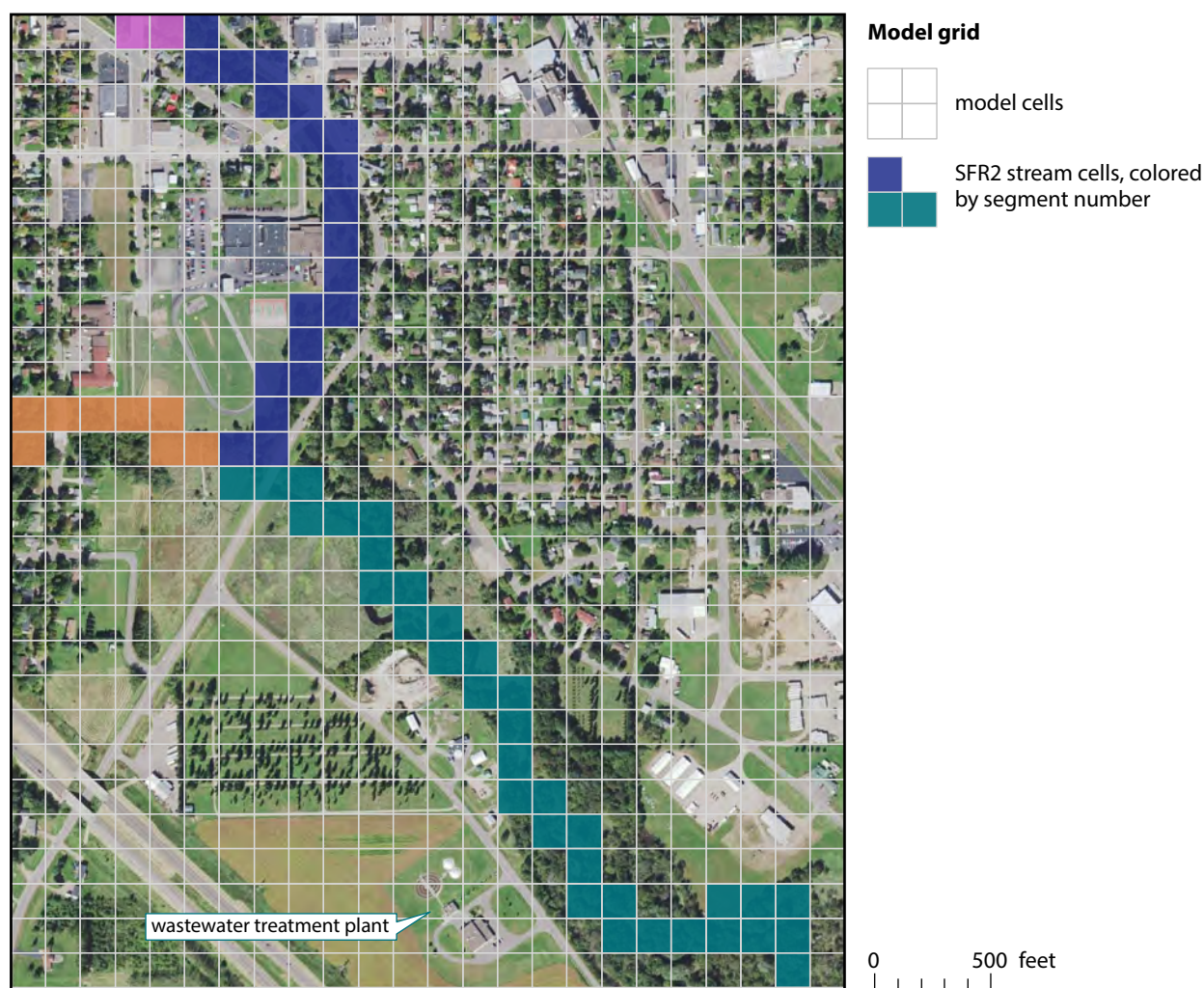
Figure 20. Example MODFLOW grid near the city of Bloomer, Wisconsin. Model cells are 150 ft on each side, colored cells are simulated stream segments.
