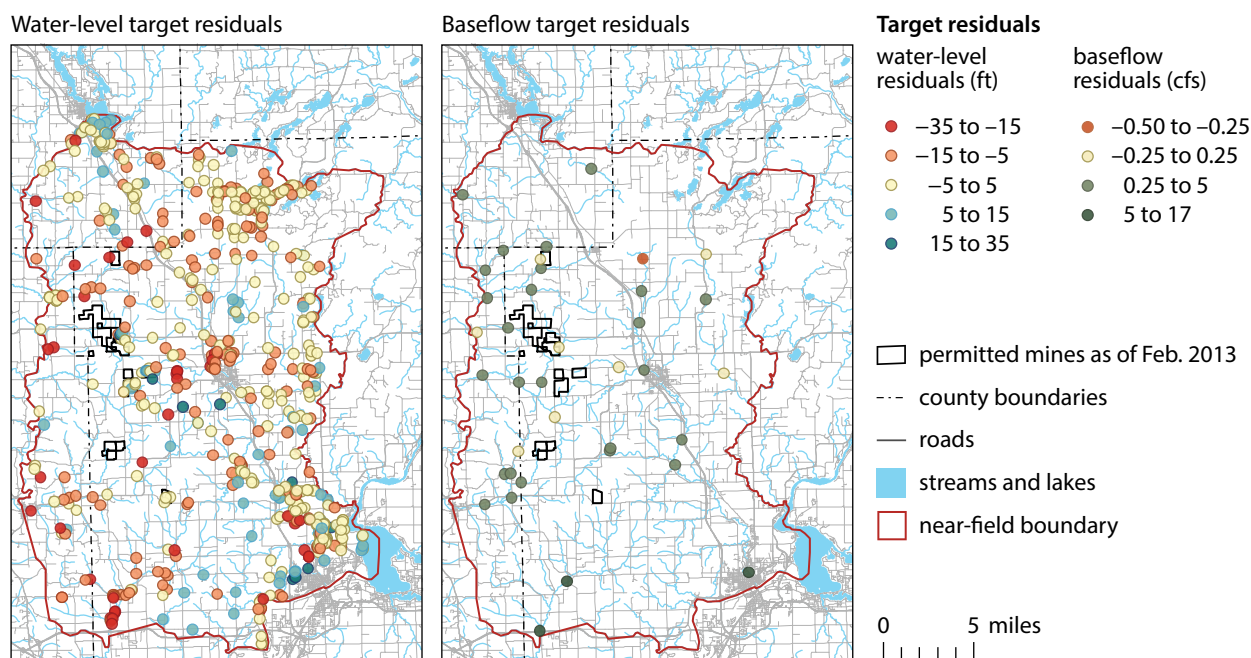
Figure 28. Target residuals. Negative residuals represent simulated results larger than target values; positive residuals represent simulated results smaller than target values.
