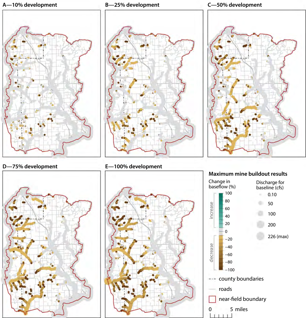
Figure 35. Percent baseflow change due to simultaneous mine development at different percentages of the minable Wonewoc resource.
