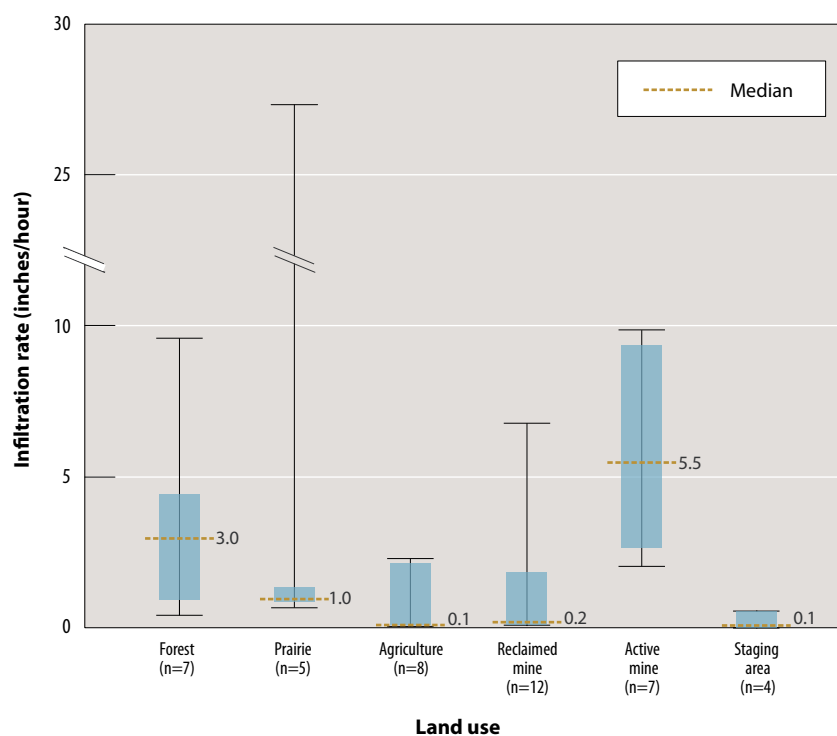
Figure 13. Infiltration rate, by land use. Vertical lines (“whiskers”) show minimum and maximum values, boxes show upper and lower quartiles, and dashed lines show medians.
