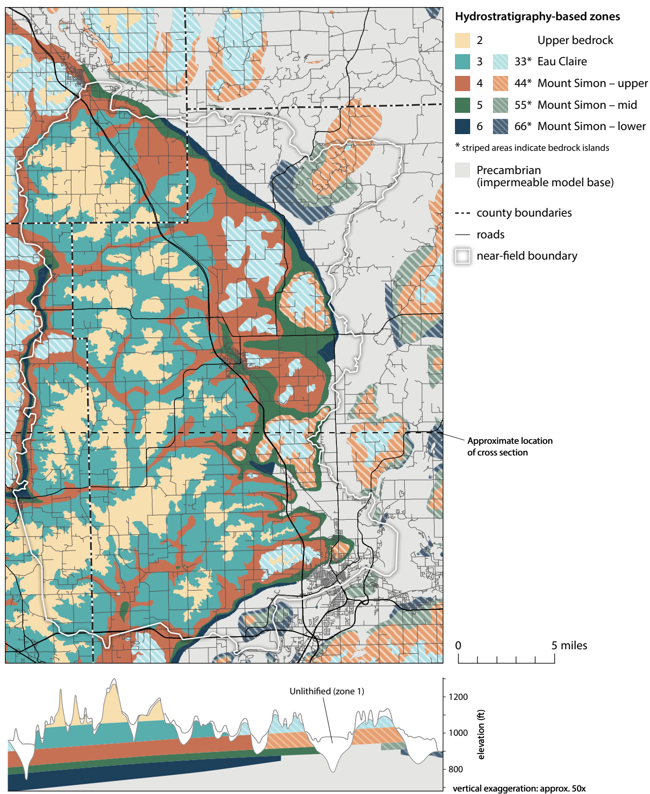
Figure 21. Hydrostratigraphic zones used to calibrate hydraulic conductivity. All zones represent areas where the associated bedrock is at least 2-ft thick. Zone 1, unlithified deposits, covers the entire model and is not shown in the map.
