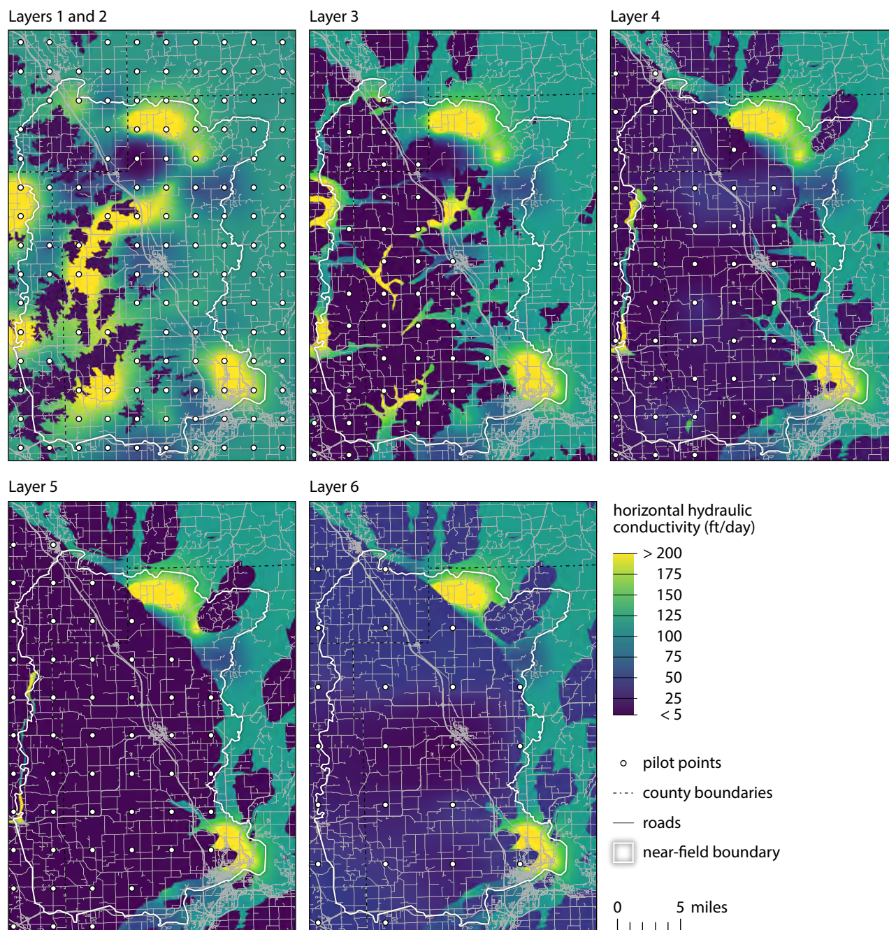
Figure 26. Calibrated horizontal hydraulic conductivity, by model layer. Layers 1 and 2 are combined because they have the same hydraulic conductivity values. Layer thickness is 2 ft wherever a unit is absent within a model layer.
