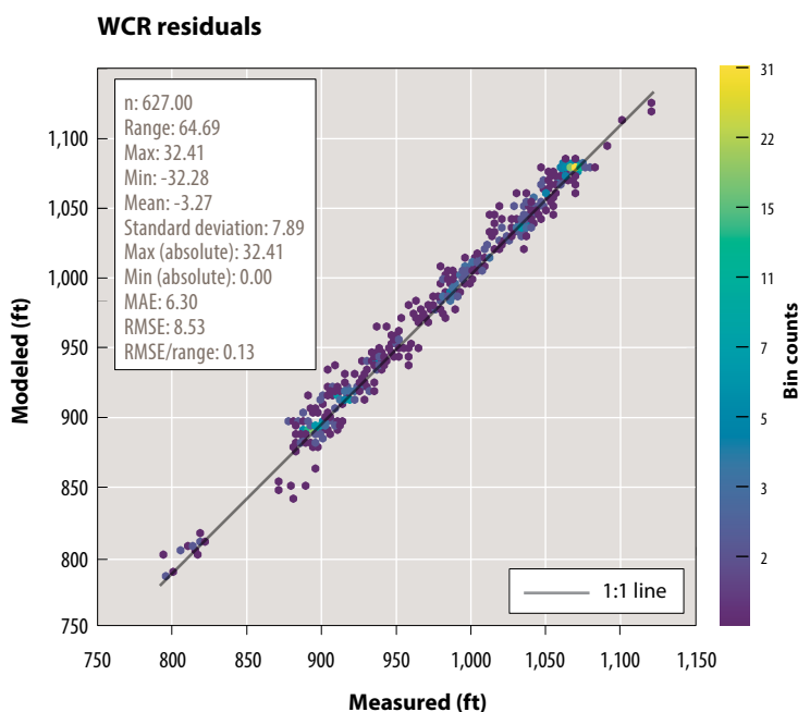
Figure 31. WCR residuals.
