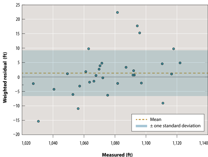
Figure 30. Mine residuals, weighted.
