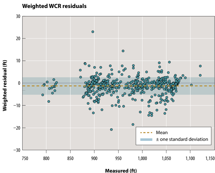
Figure 32. WCR residuals, weighted.
